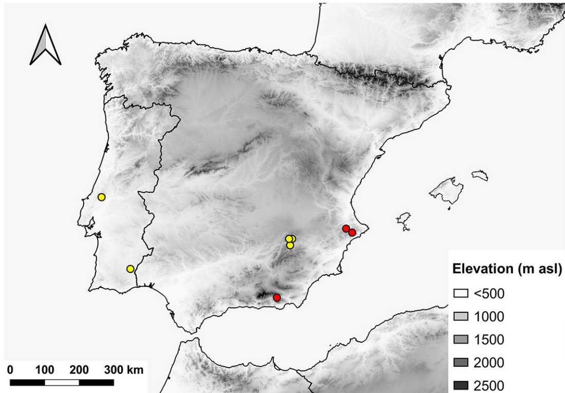
Supplementary figure 4. Ibero-Balearic distribution of E. gibbosus . New records, red circle. Literature records, yellow circle. Source: Aguado-Aranda et al. (2024).
