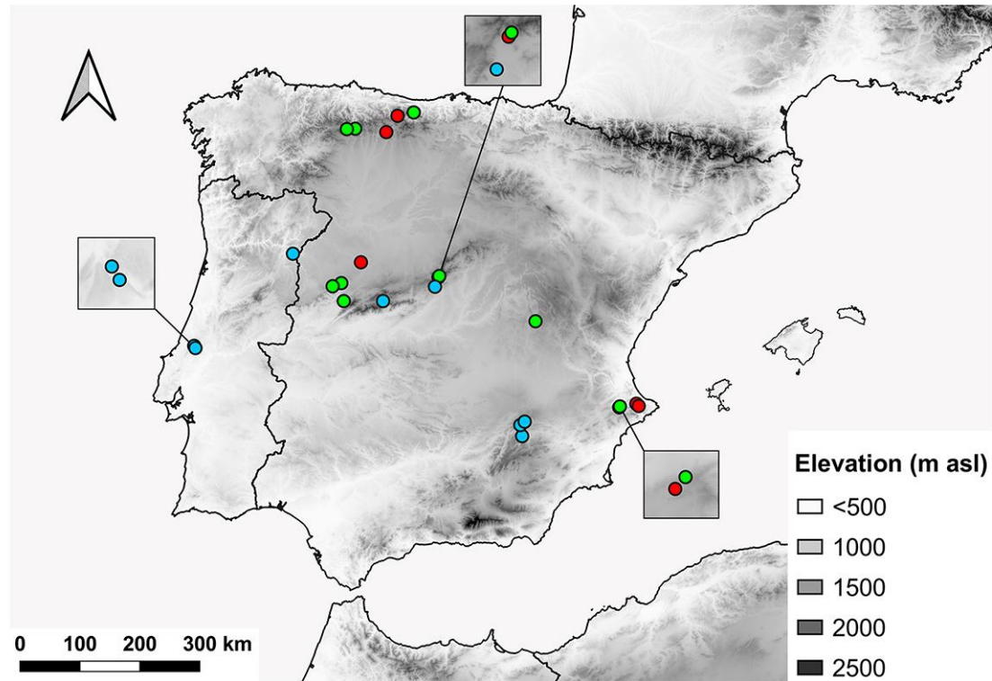
Supplementary figure 3. Ibero-Balearic distribution of E. sulcitibius . New records, red circle. Confirmed literature records, green circle. Unconfirmed literature records, blue circle. Source: Aguado-Aranda et al. (2024).
